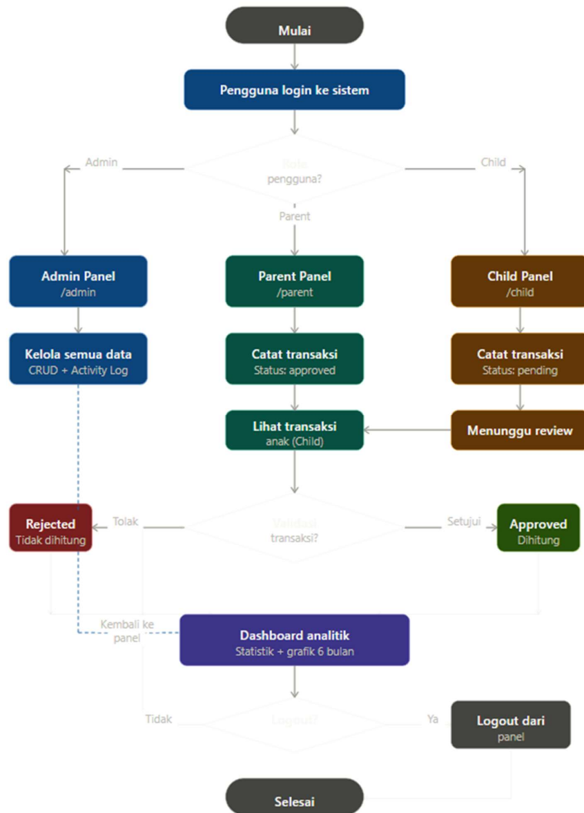
Gambar 2. Flowchart Sistem DompetKuu — Alur Login Multi-Panel & Approval Workflow
